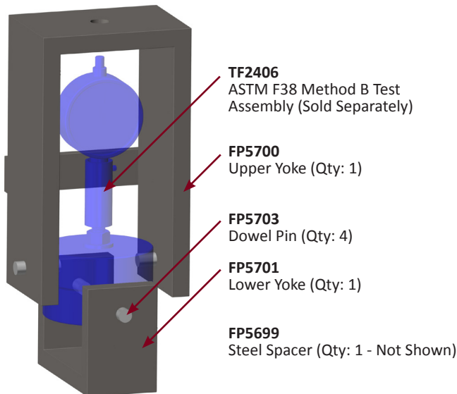
ASTM F38 Method B Bolt Calibration Apparatus
