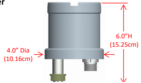
Figure 1. MS2600E Dimensions
