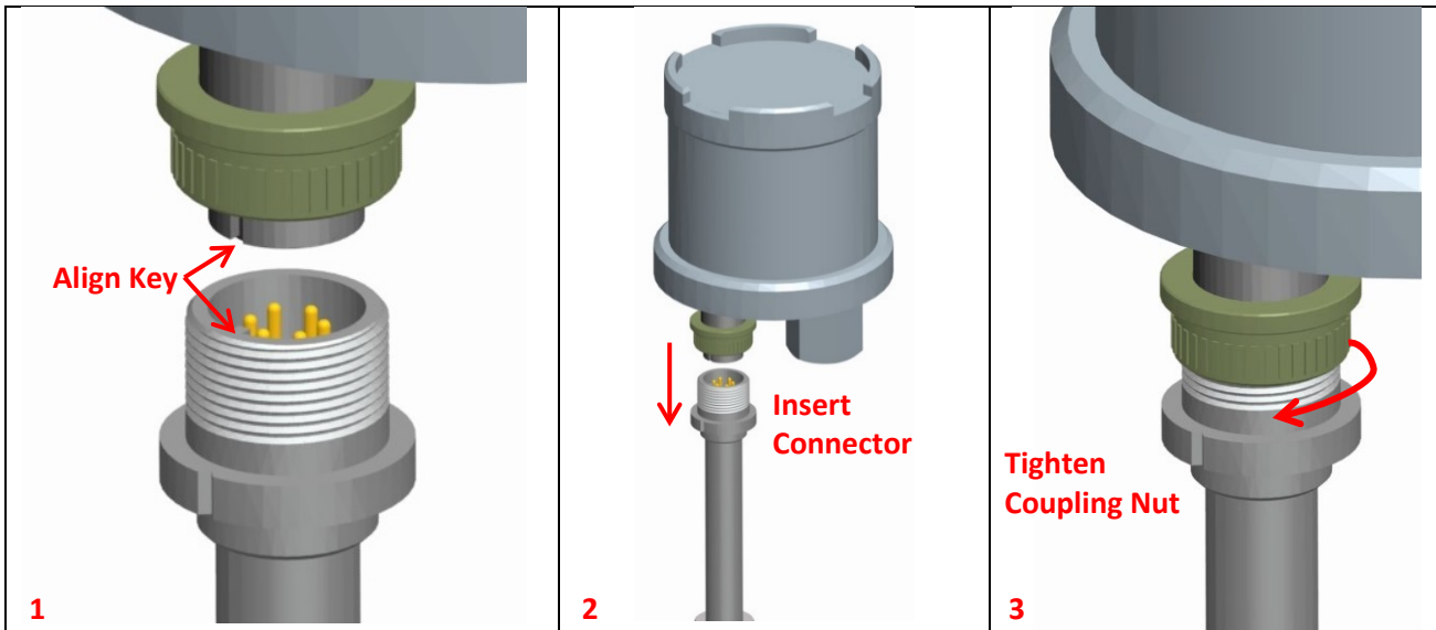
Figure 2. MS2600E Direct Mount Installation
